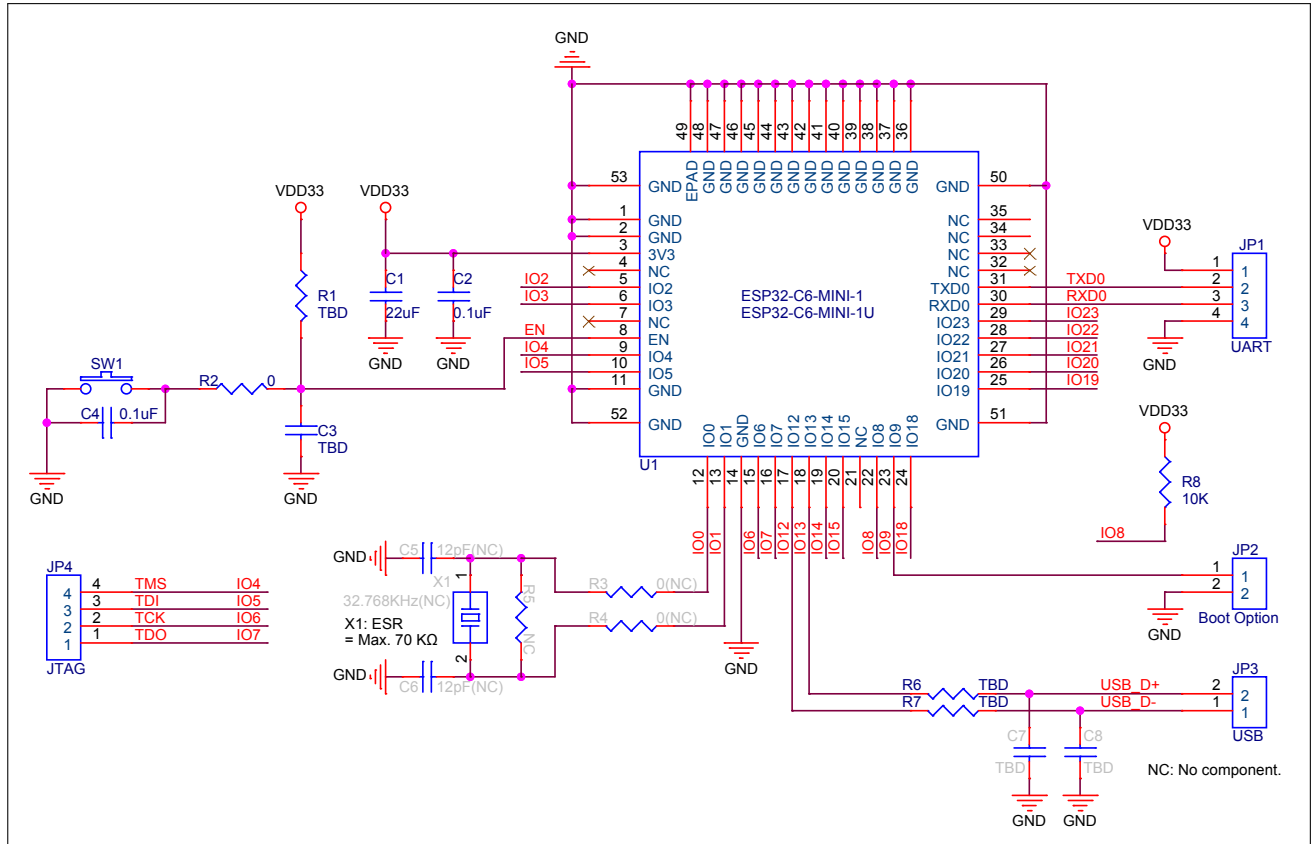
Figure 9-1. Peripheral Schematics
