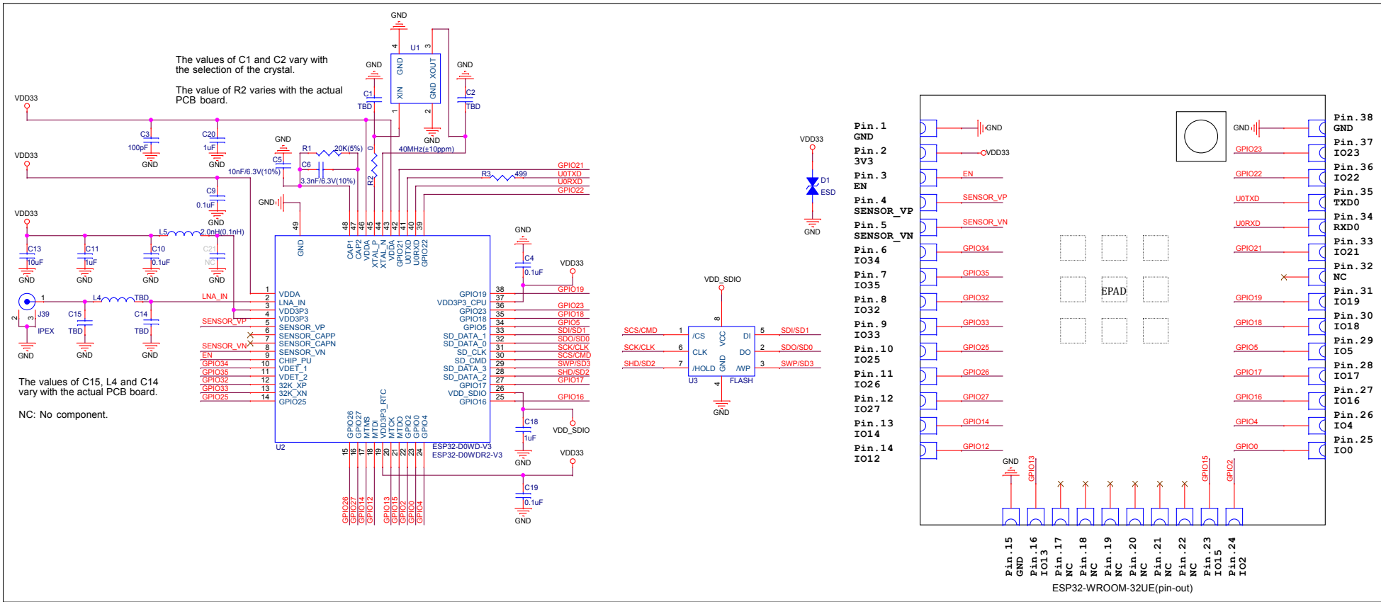
Figure 7: ESP32-WROOM-32UE Schematics
